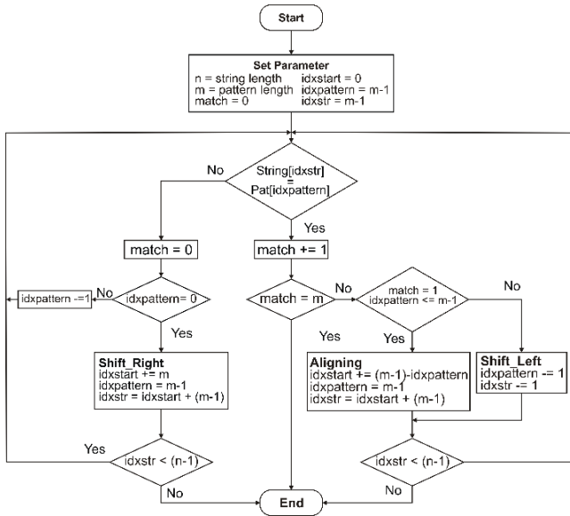
Figure 2. Boyer-Moore string matching flowchart
