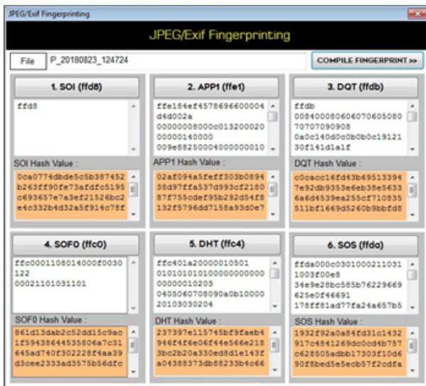
Figure 9. segment content acquisition and hashing
